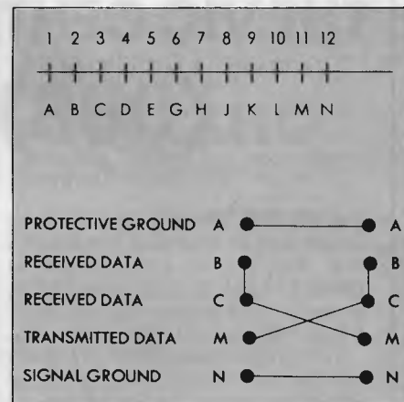
Fig 1 User port pinout (see page 152 of the Owners Manual)
